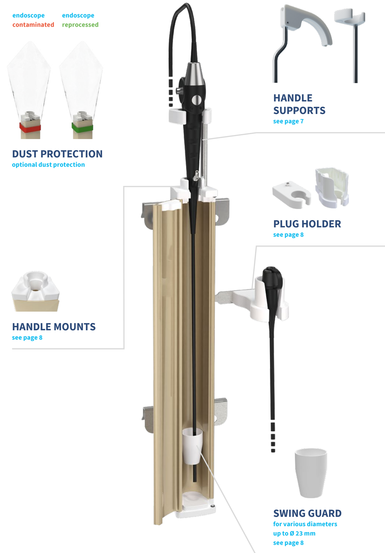
Figure shows thermo-disinfectable protector (versions 500 and 700 mm)
